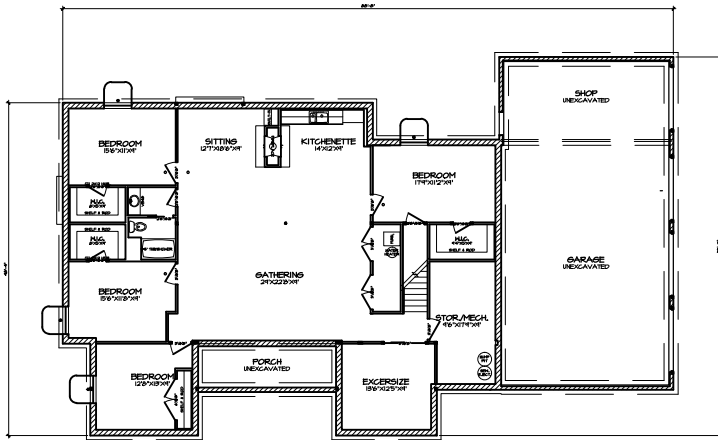
FOUNDATION PLAN A-A
