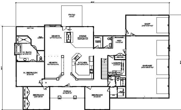
FIRST FLOOR PLAN A-A
